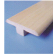
T-molding piece size:2400x46x10(mm) package:20 pieces/carton
